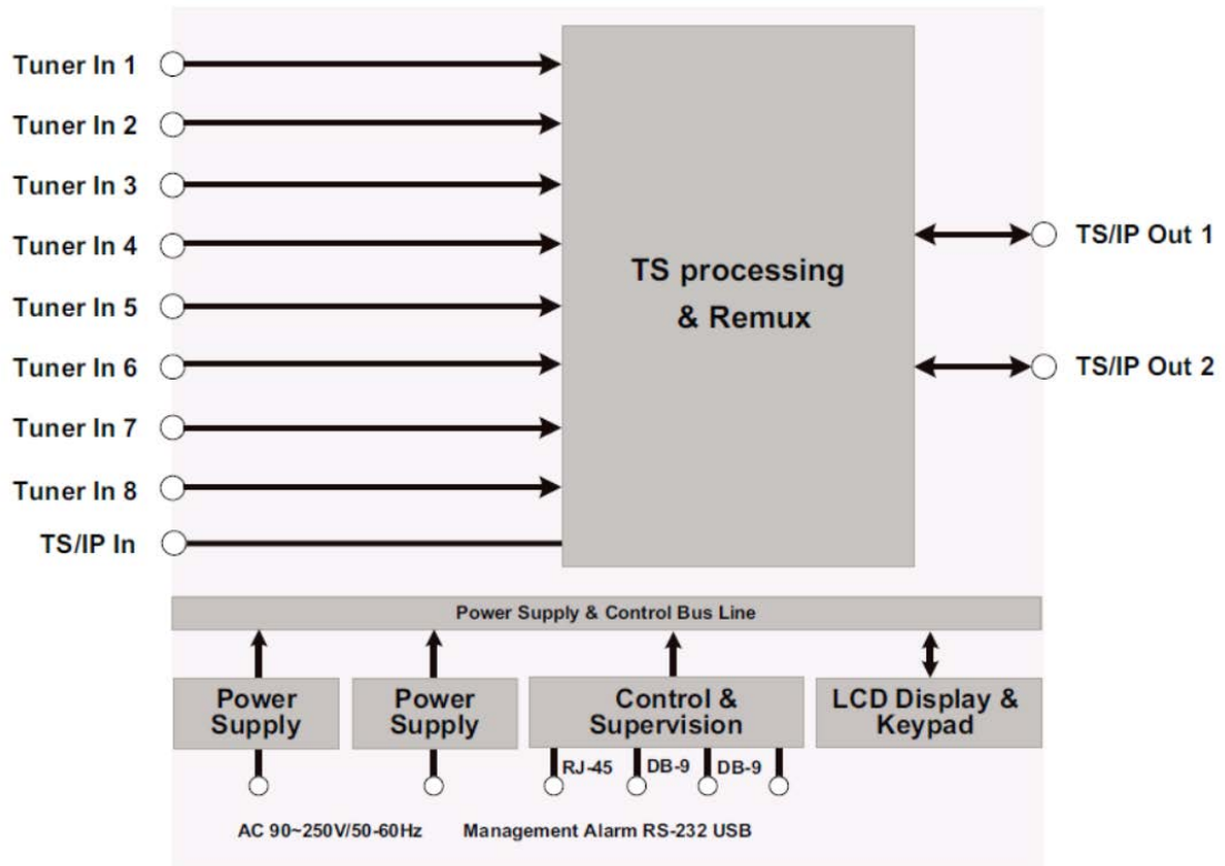
WHX-9000D Functional Block Diagram
