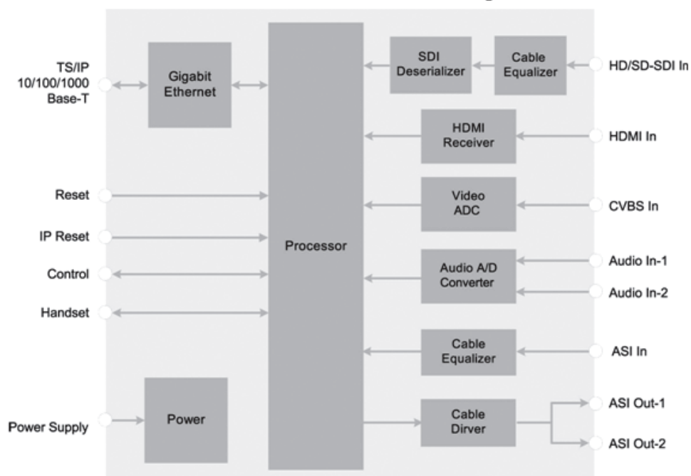
WDH-1530EC Functional Block Diagram
